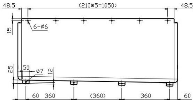
Rear View - UR2
