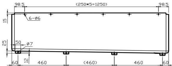
Rear View - UR5
