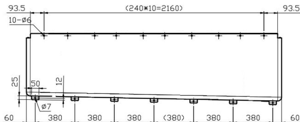
Rear View - UR6
