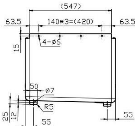
Rear View - UR4
