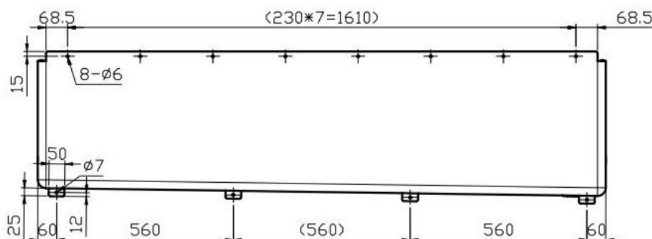
Rear View - UR3
