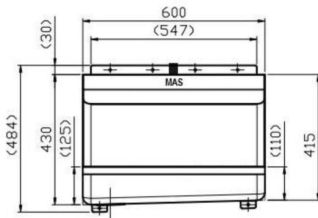
Front View - UR4
