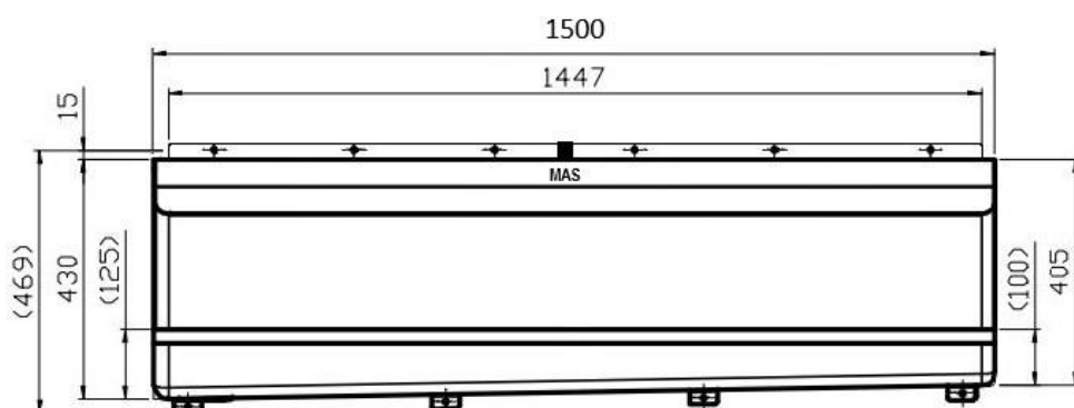
Front View - UR5
