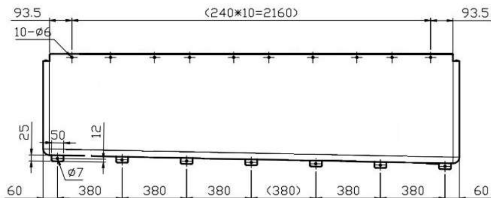
Rear View - UR6
