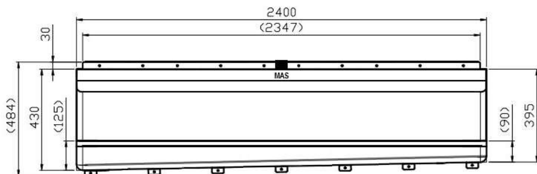
Front View - UR6
